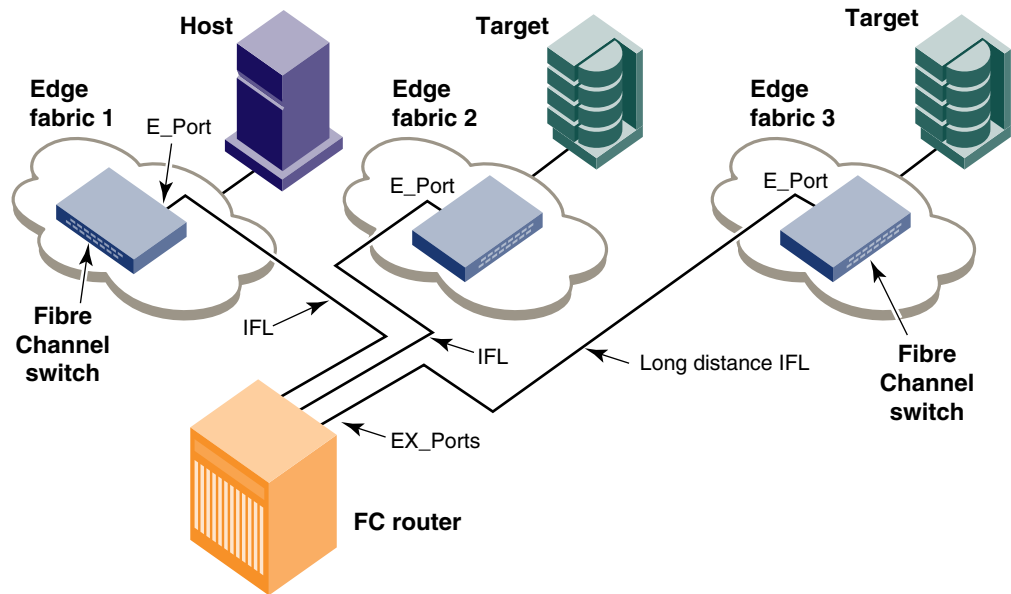
FIGURE 68 A metaSAN with inter-fabric links
